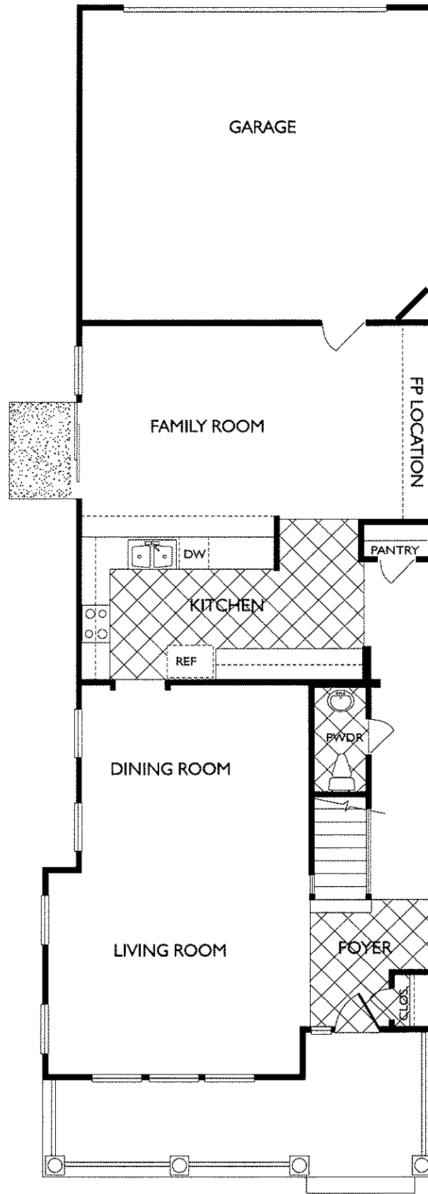
FIRST FLOOR PLAN MODEL-KFF-B-1070 MODEL-KFF-B-1071
